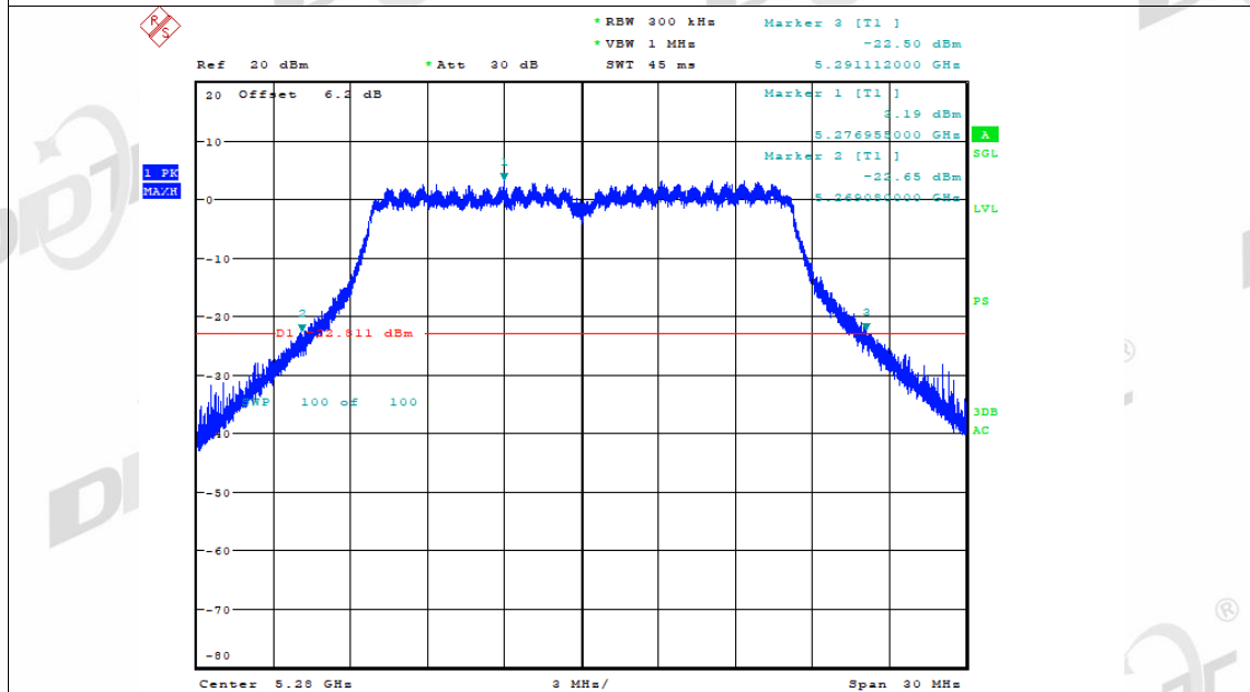
-26dB Bandwidth NVNT a 5280MHz Ant2
