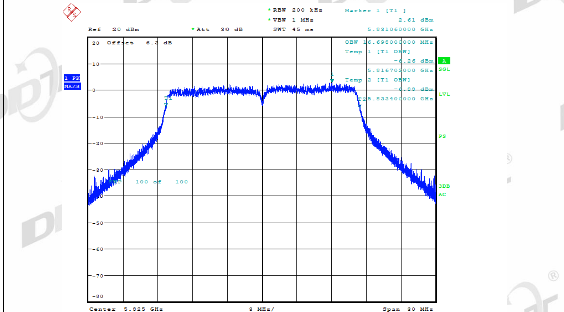
OBW NVNT a 5825MHz Ant1
