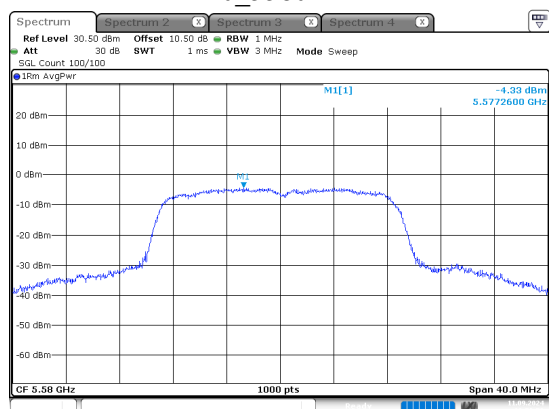
n20_5580MHz
