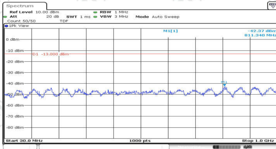
Band4-5MHz-16QAM-20375-1RB#0-Range1:30~1000MHz
