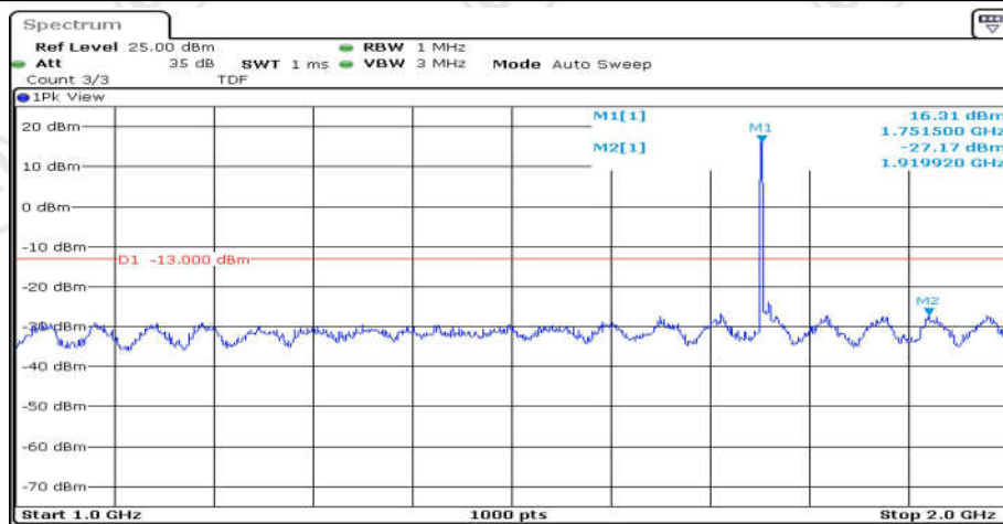
Band4-5MHz-16QAM-20375-1RB#0-Range2:1000~2000MHz
