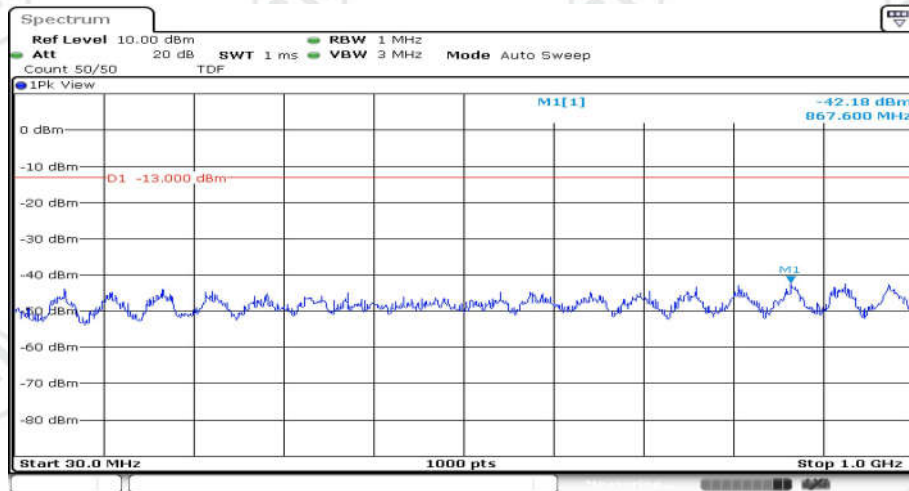
Band4-3MHz-16QAM-19965-1RB#0-Range1:30~1000MHz
