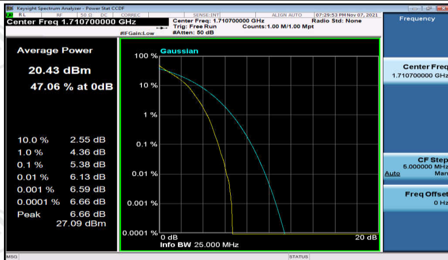
Band4-1.4MHz-QPSK-19957-6RB#0
