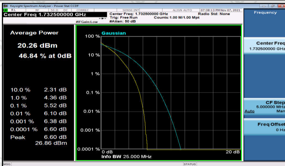
Band4-5MHz-QPSK-20375-1RB#0
