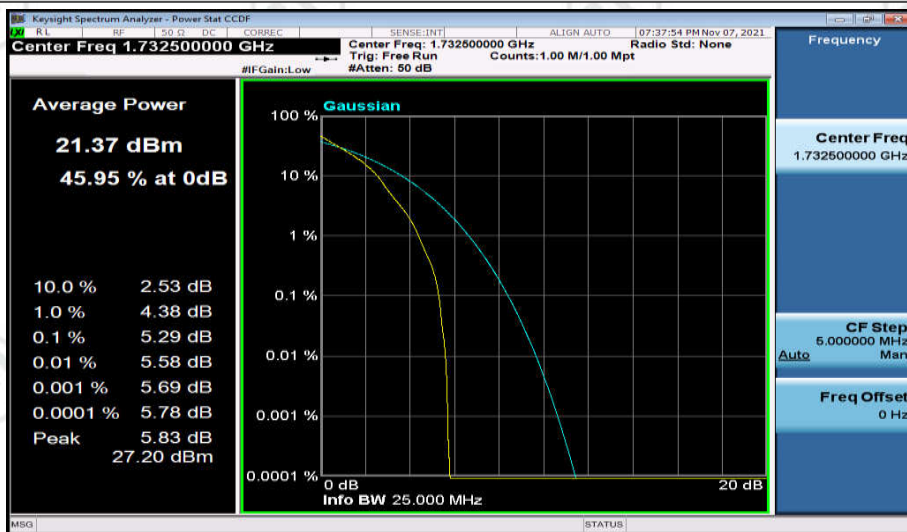
Band4-5MHz-QPSK-20175-25RB#0
