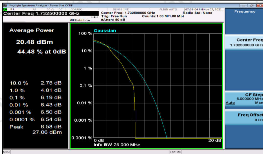
Band4-5MHz-16QAM-20175-25RB#0
