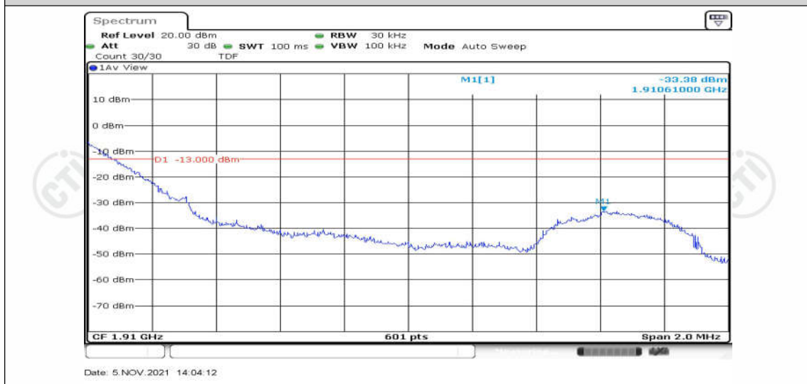
Band2-1.4MHz-QPSK-19193-1RB#5
