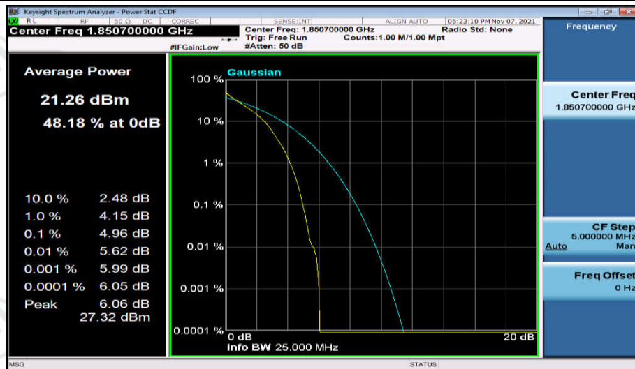
Band2-1.4MHz-QPSK-18607-6RB#0
