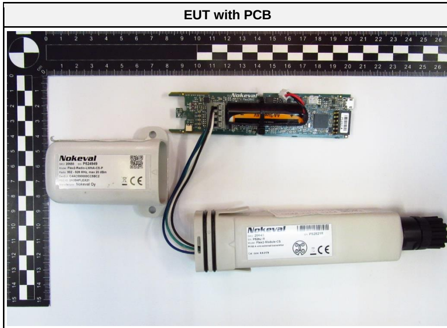
EUT with Radio Module
