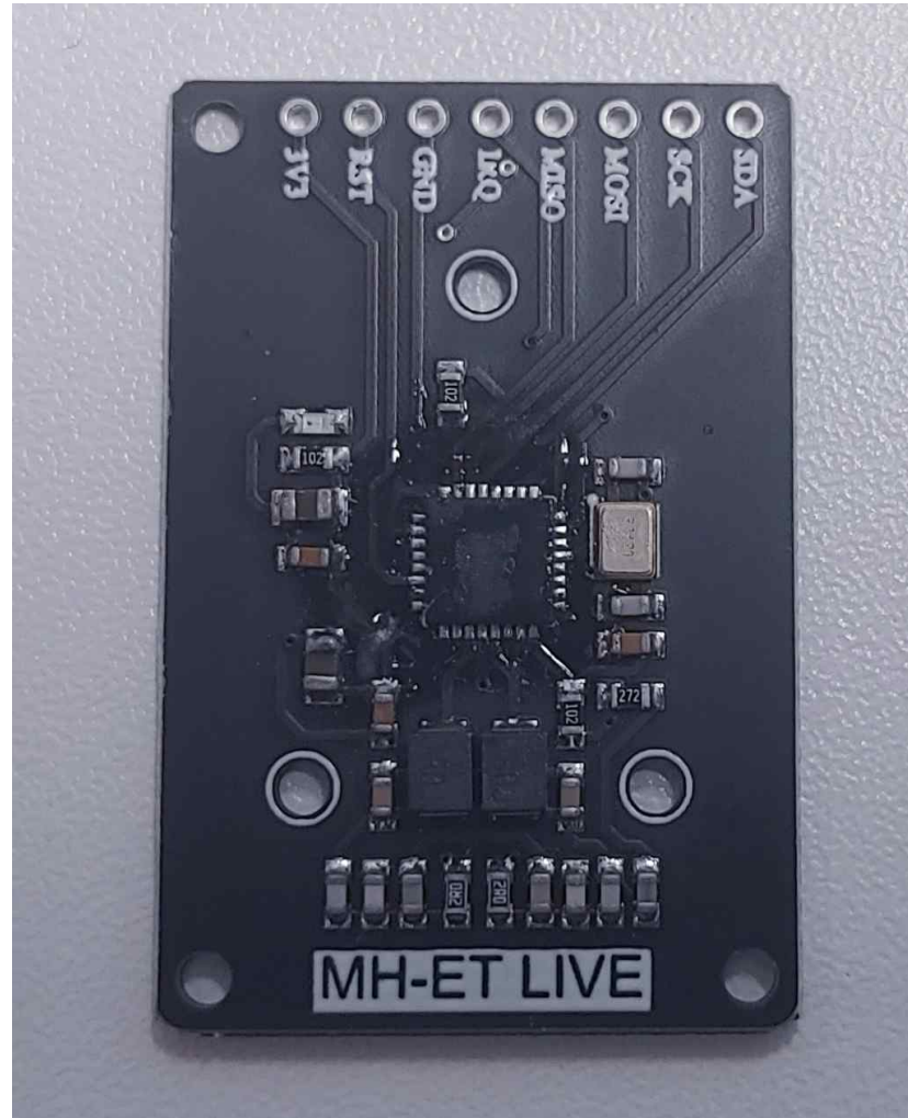
[NFC board(Top)]
