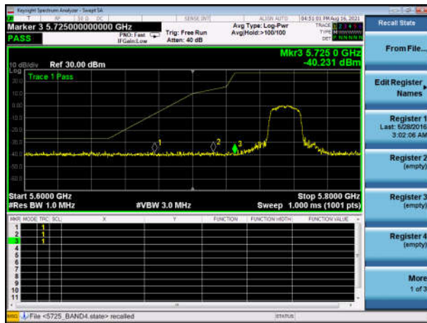
U-NII-3 ,Plot 1,Band Edge-802.11ac(80 MHz),5775MHz,Ant1 Left side band
