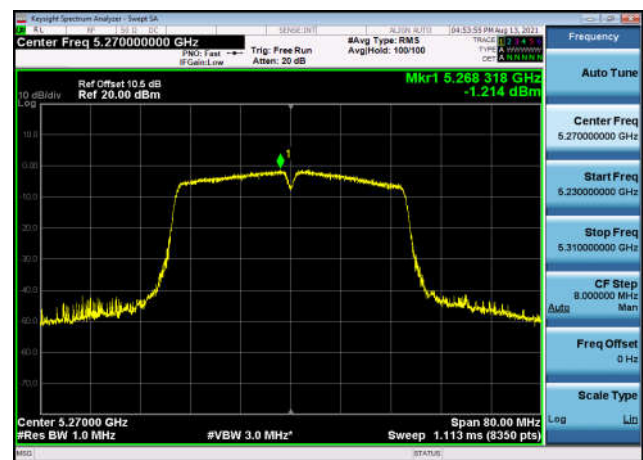
U-NII-2a Power spectral density-802.11 1n(40MHz),5270MHz,Ant1
