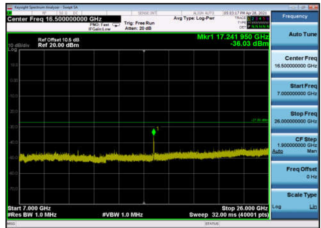
U-NII-3 ,Plot 4,7000MHz~26000MHz-802. 11a(20MHz),5825MHz,Ant1
