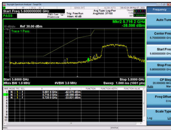
U-NII-3 ,Plot 1,Band Edge-802.11ac(80 MHz),5775MHz,Ant1 Left side bandedge
