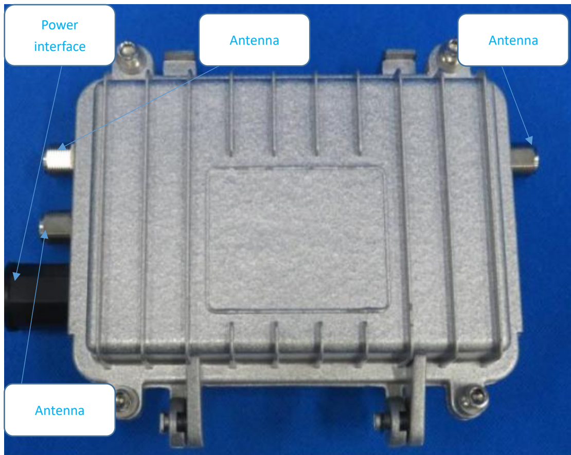
Figure 2-1 PISCES P100 appearance
