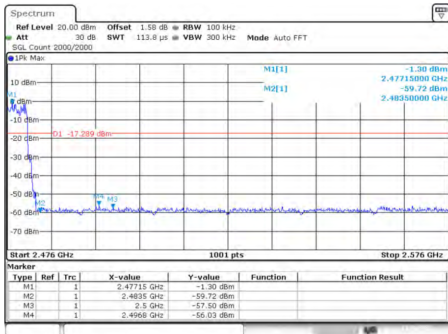
Band Edge(Hopping) NVNT 3-DH5 2480MHz Hopping Ref
