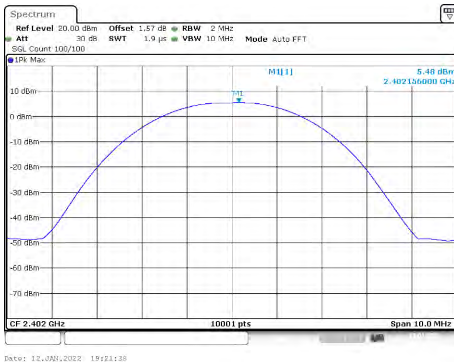
Power NVNT 1-DH5 2402MHz
