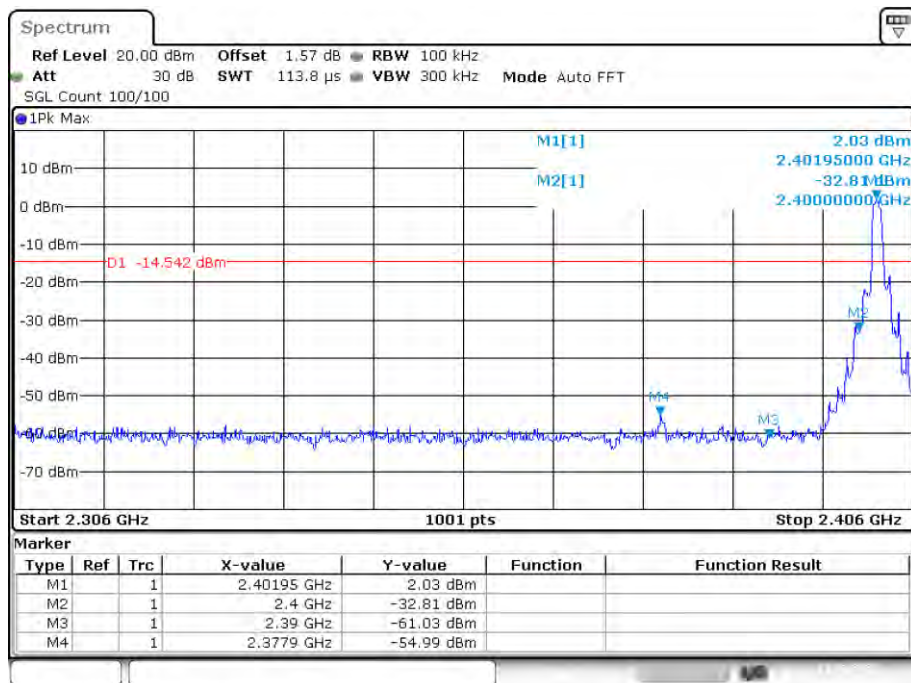
Band Edge NVNT 3-DH5 2402MHz No-Hopping Emission
