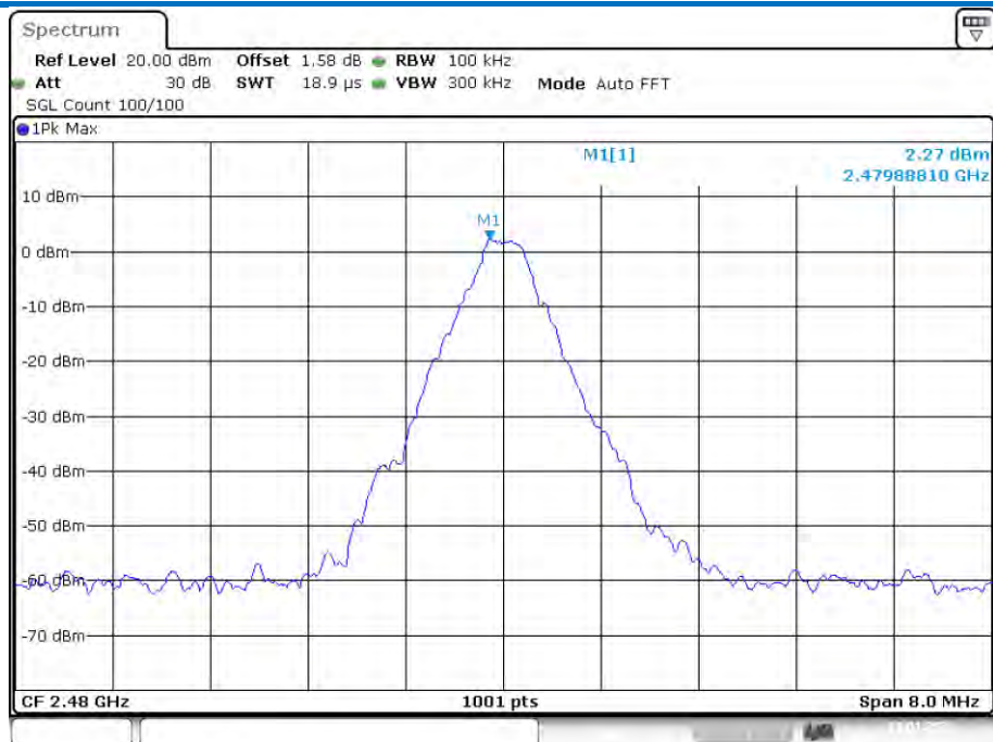
Band Edge NVNT 1-DH5 2480MHz No-Hopping Ref
