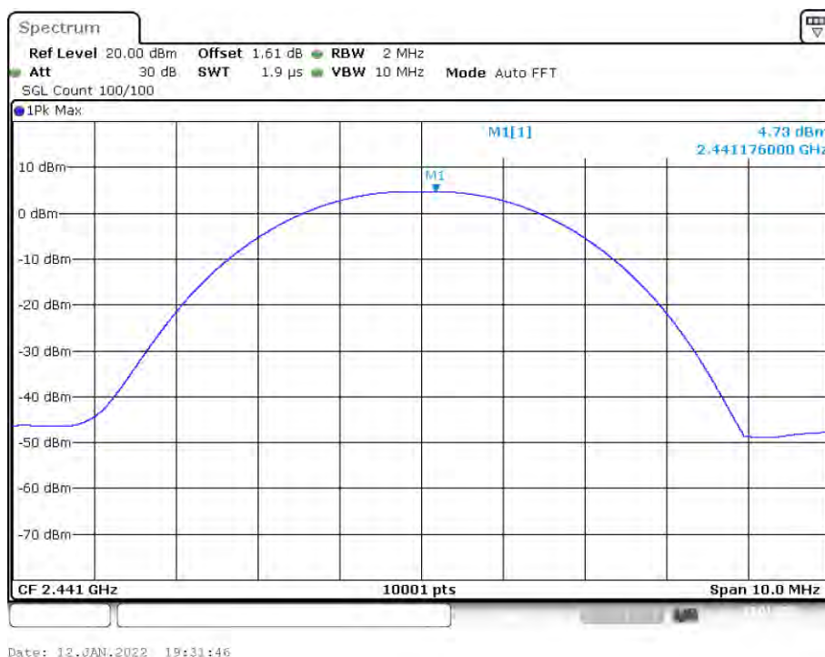
Power NVNT 1-DH5 2441MHz
