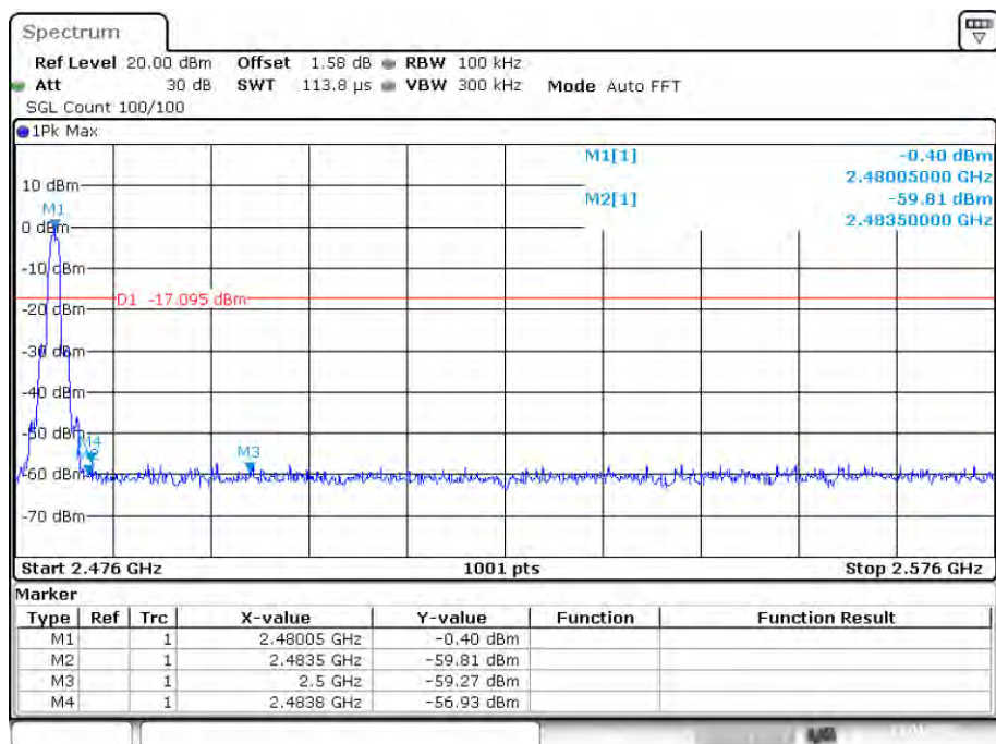
Band Edge NVNT 2-DH5 2480MHz No-Hopping Ref
