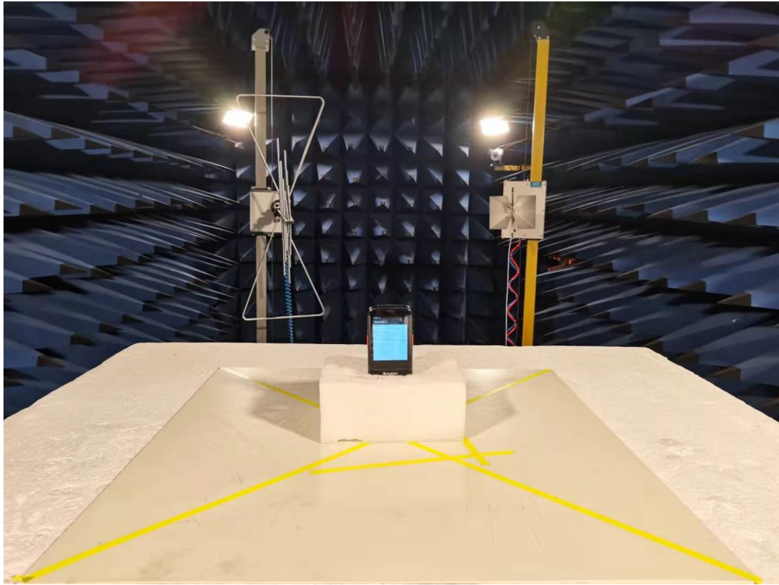
Radiated Spurious Emission below 18GHz
