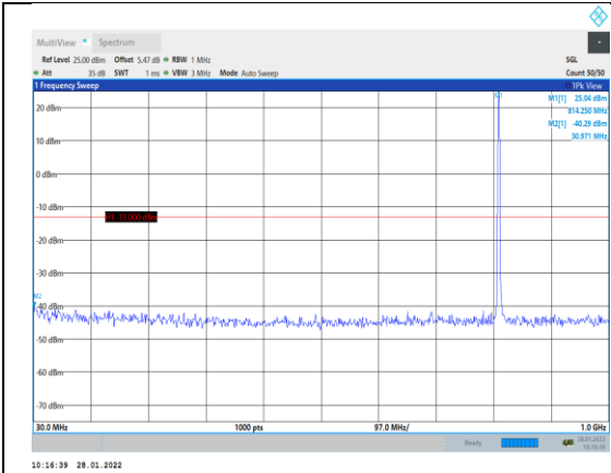
Band26-1.4MHz-QPSK-26697-1RB#0-Range :30~1000MHz
