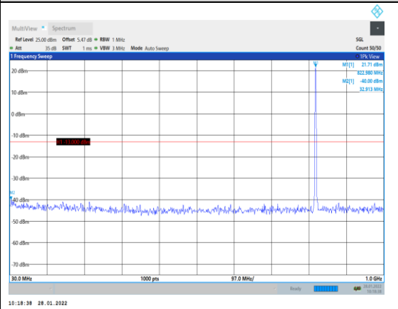
Band26-1.4MHz-QPSK-26783-1RB#0-Range1 :30~1000MHz
