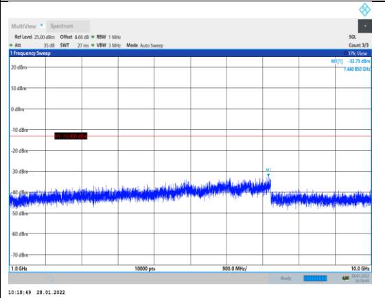
Band26-1.4MHz-QPSK-26783-1RB#0-Range2 :1000~10000MHz
