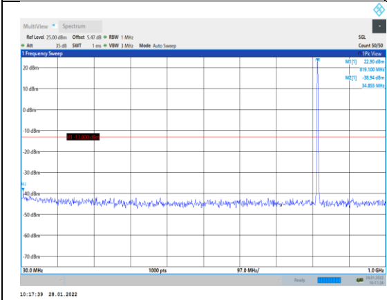
Band26-1.4MHz-QPSK-26740-1RB#0-Range :30~1000MHz
