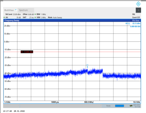
Band26-1.4MHz-QPSK-26740-1RB#0-Range2 :1000~10000MHz
