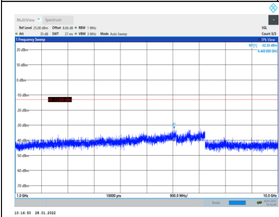
Band26-1.4MHz-QPSK-26697-1RB#0-Range :1000~10000MHz
