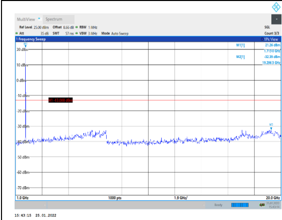
Band4-10MHz-16QAM-20000-1RB#0-Range2: 1000~20000MHz
