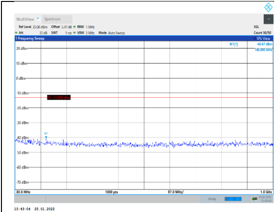
Band4-10MHz-16QAM-20000-1RB#0-Range1: 30~1000MHz
