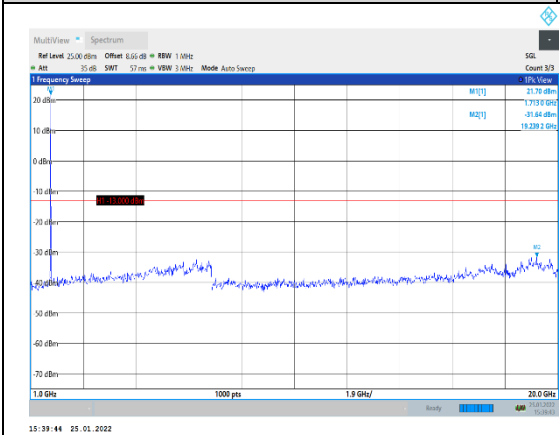
Band4-5MHz-16QAM-19975-1RB#0-Range2: 000~20000MHz
