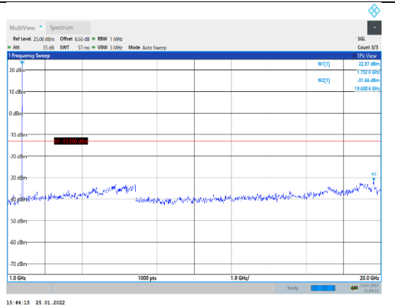
Band4-10MHz-16QAM-20175-1RB#0-Range2: 1000~20000MHz
