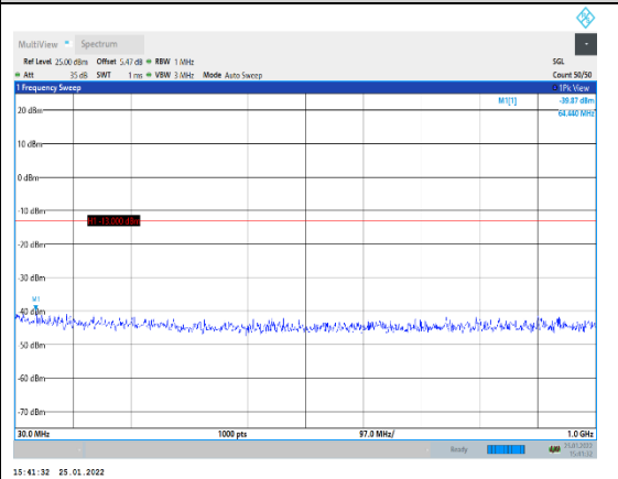
Band4-5MHz-16QAM-20375-1RB#0-Range1: 3 0~1000MHz
