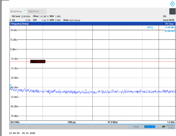
Band4-10MHz-16QAM-20175-1RB#0-Range2: 30~1000MHz
