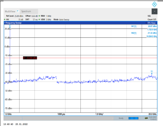
Band4-5MHz-16QAM-20175-1RB#0-Range2: 1 000~20000MHz
