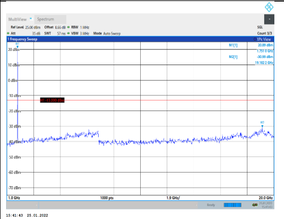
Band4-5MHz-16QAM-20375-1RB#0-Range2: 1 000~20000MHz
