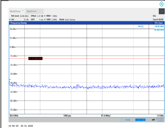
Band4-5MHz-16QAM-20175-1RB#0-Range1: 0~1000MHz
