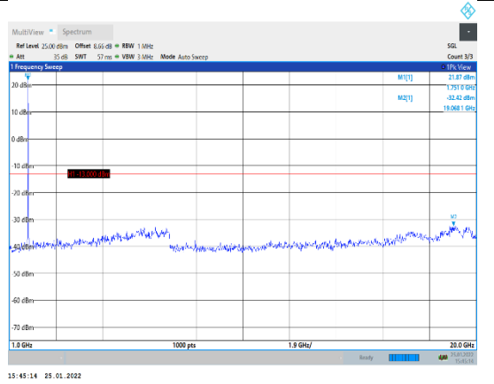
Band4-10MHz-16QAM-20350-1RB#0-Range2: 1000~20000MHz
