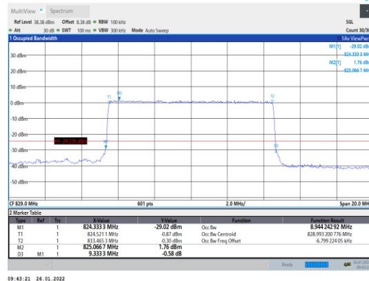
Band5-10MHz-16QAM-20450-50RB#0
