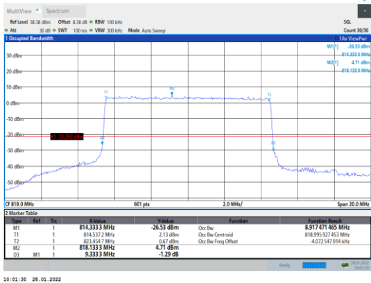
Band26-10MHz-QPSK-26740-50RB#0
