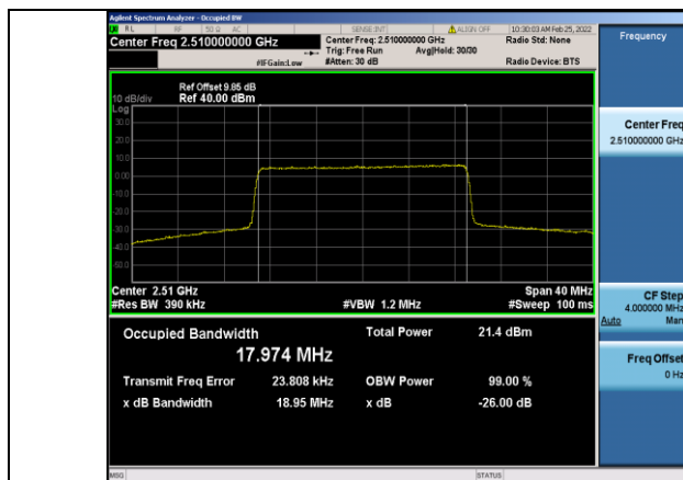
Band7-20MHz-QPSK-20850-100RB#0
