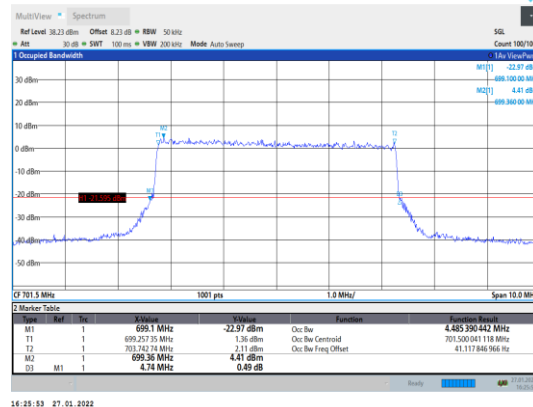
Band12-5MHz-16QAM-23035-25RB#0
