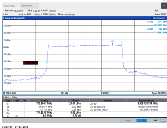
Band12-10MHz-QPSK-23130-50RB#0
