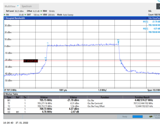
Band12-5MHz-16QAM-23095-25RB#0
