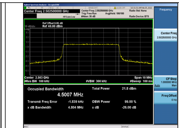
Band7-5MHz-16QAM-20775-25RB#0
