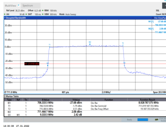
Band12-10MHz-16QAM-23130-50RB#0
