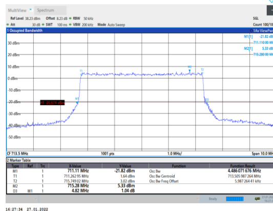
Band12-5MHz-16QAM-23155-25RB#0
