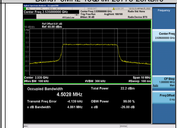
Band7-5MHz-16QAM-21100-25RB#0
