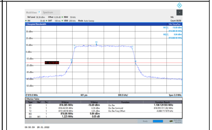
Band26-1.4MHz-16QAM-26740-6RB#0
