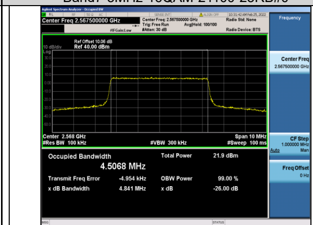
Band7-5MHz-16QAM-21425-25RB#0
