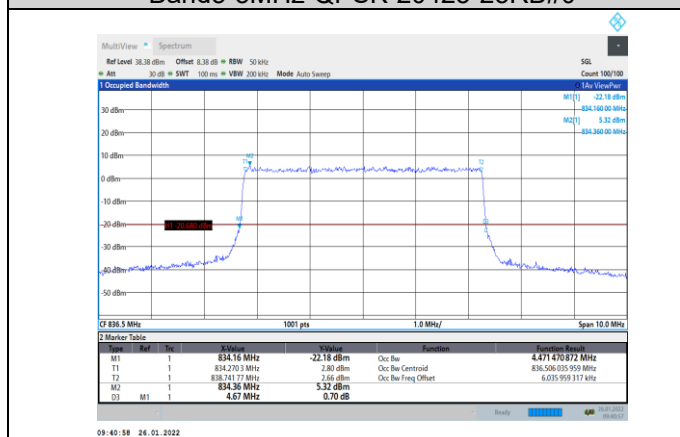
Band5-5MHz-QPSK-20525-25RB#0
