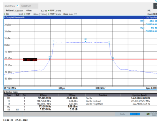
Band12-1.4MHz-16QAM-23173-6RB#0
