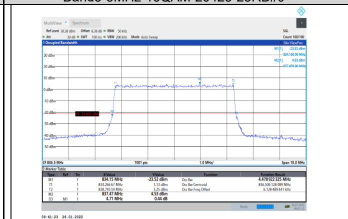
Band5-5MHz-16QAM-20525-25RB#0
