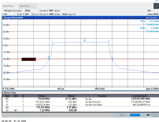
Band12-1.4MHz-QPSK-23173-6RB#0
