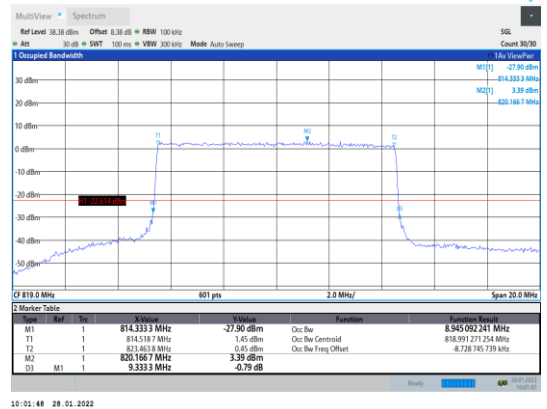
Band26-10MHz-16QAM-26740-50RB#0
