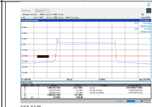
Band2-10MHz-16QAM-19150-50RB#0
