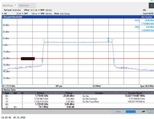
Band4-15MHz-QPSK-20025-75RB#0
