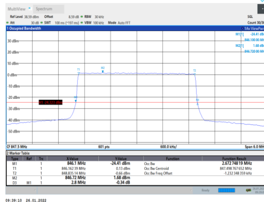
Band5-3MHz-16QAM-20635-15RB#0
