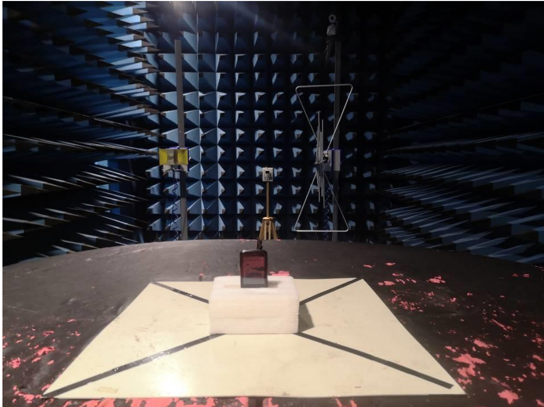
FCC Part15C Radiated Emission 18-26GHz
