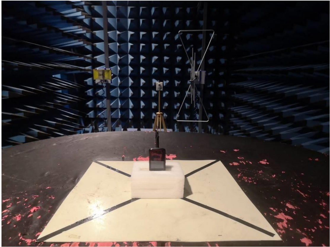
FCC Part15C Radiated Emission 26-40GHz
