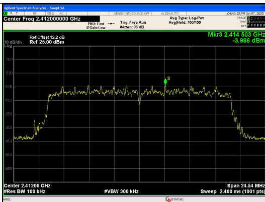
In-Band Reference Level IEEE 802.11n Channel 1 20MHz Antenna 0
