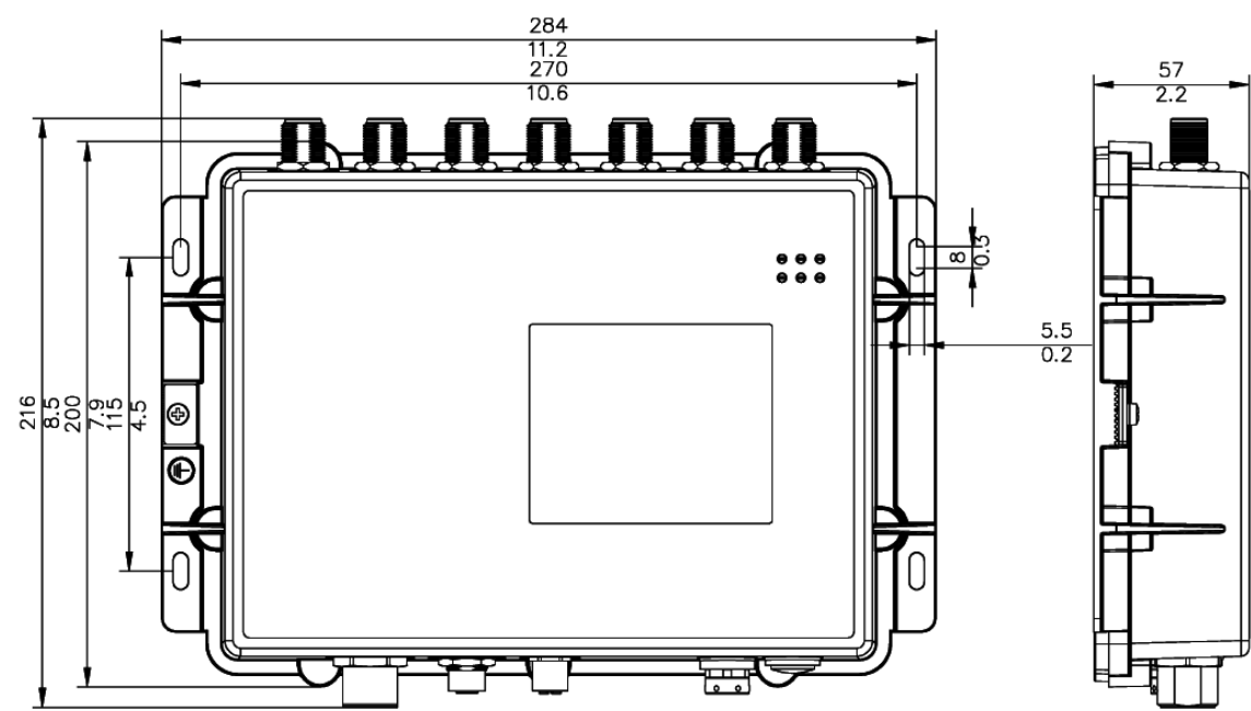
Figure 20: DAP847 dimensional measurements (unit: mm/inch)
