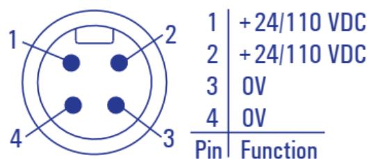
Figure 8: Pin assignment of the power supply socket
