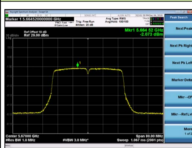
Channel 134 (5670MHz)
