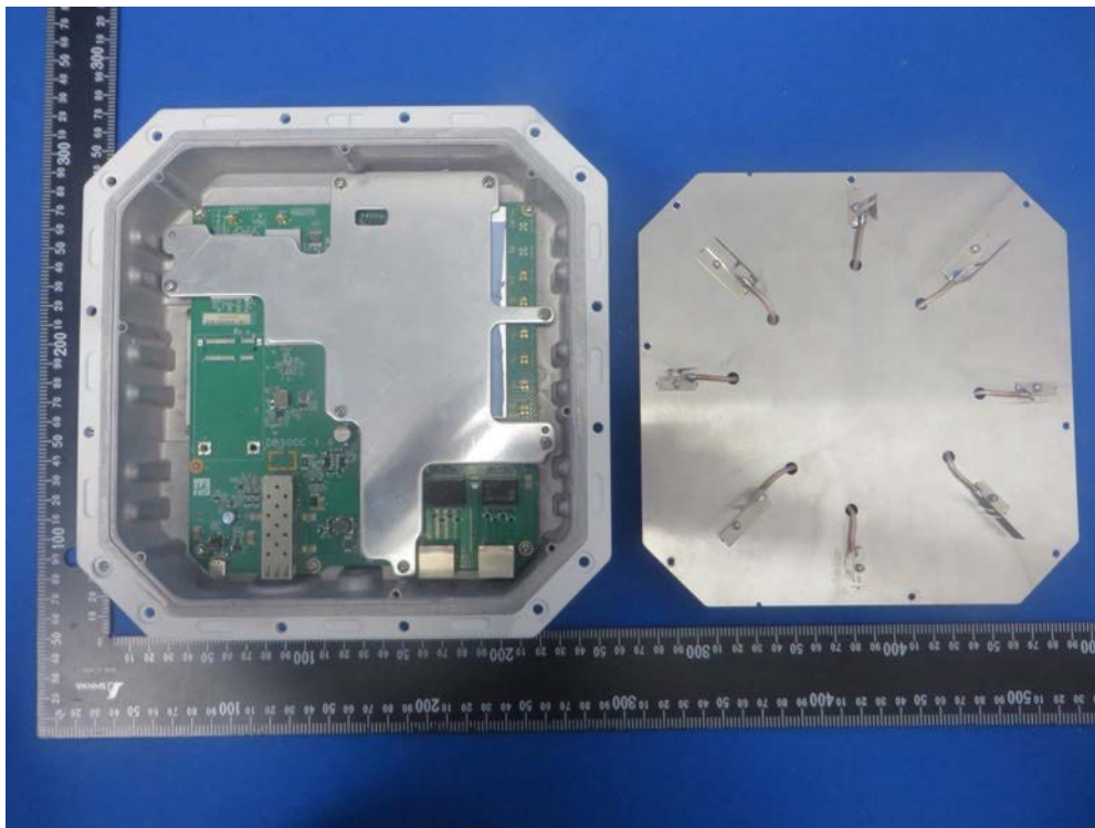
(2) EUT Photo - Original 1 st model
