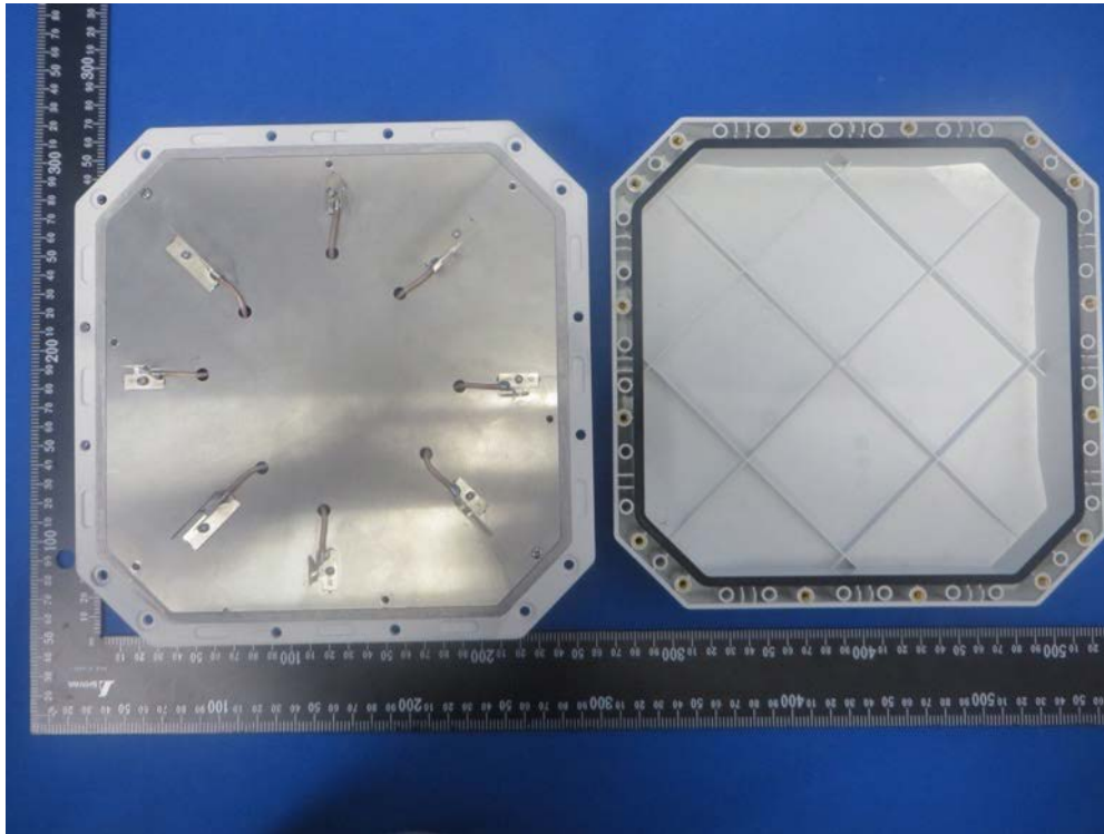
(1) EUT Photo - Original 1 st model
