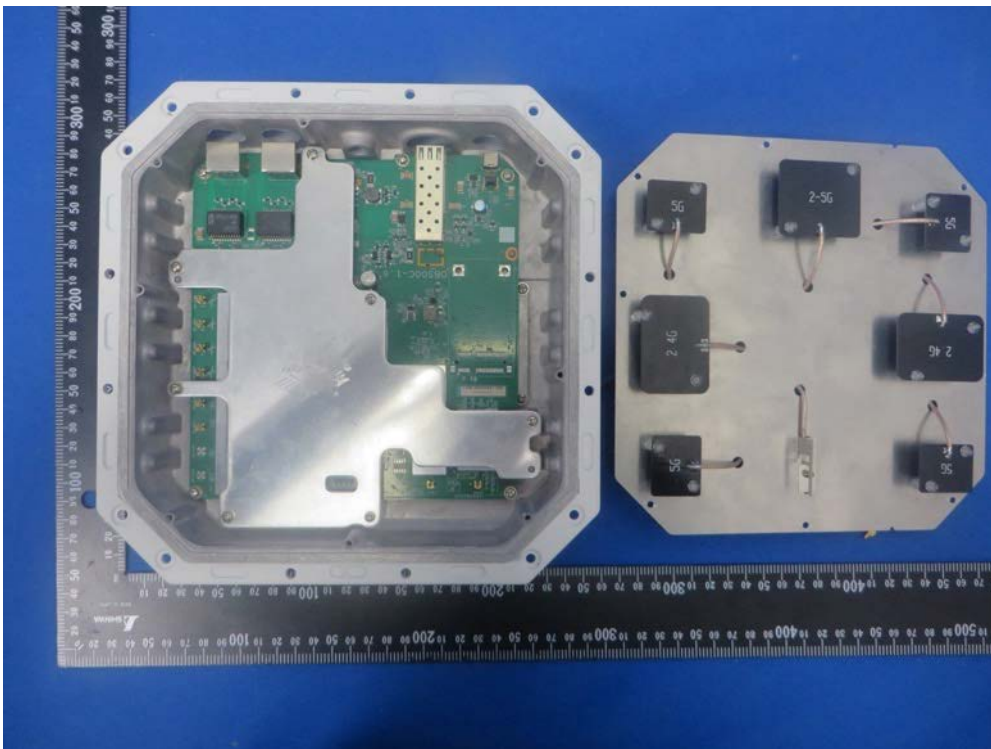
(4) EUT Photo - Original 2 nd model
