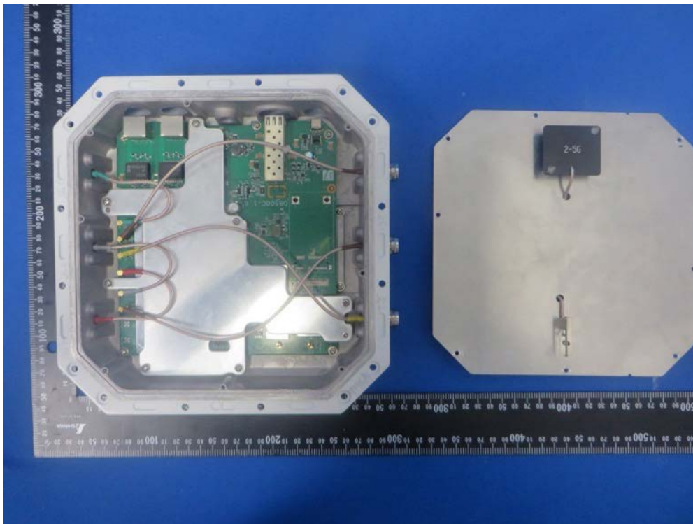
(6) EUT Photo - Original 3 rd model
