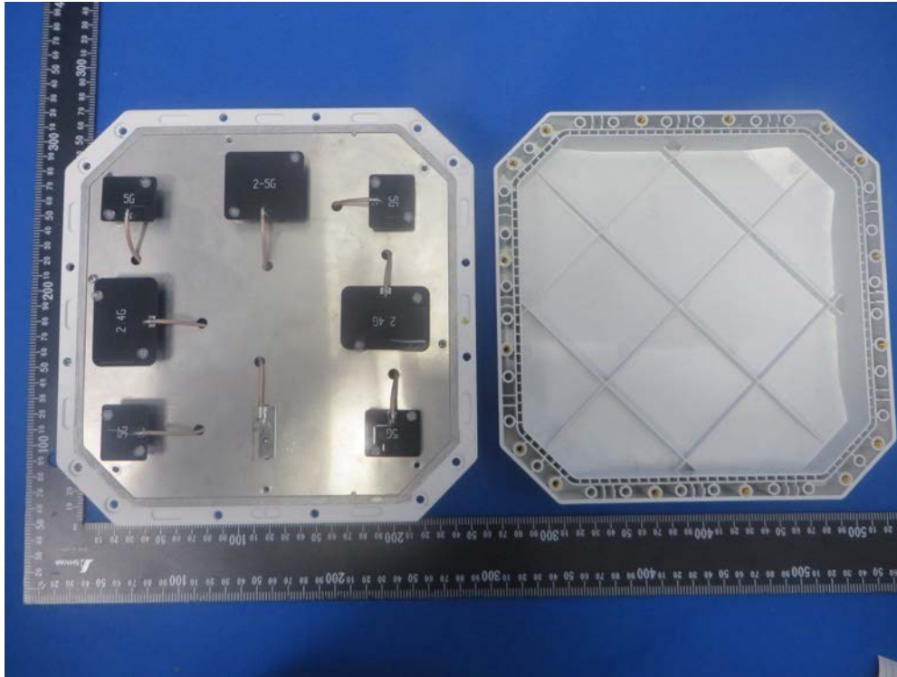
(3) EUT Photo - Original 2 nd model
