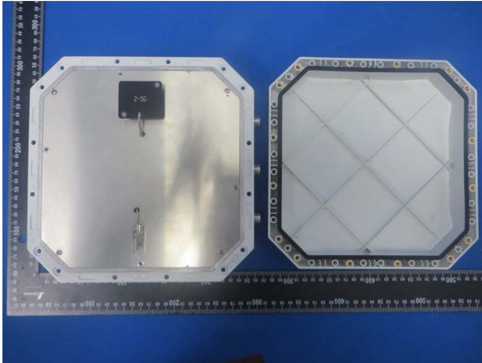
(5) EUT Photo - Original 3 rd model
