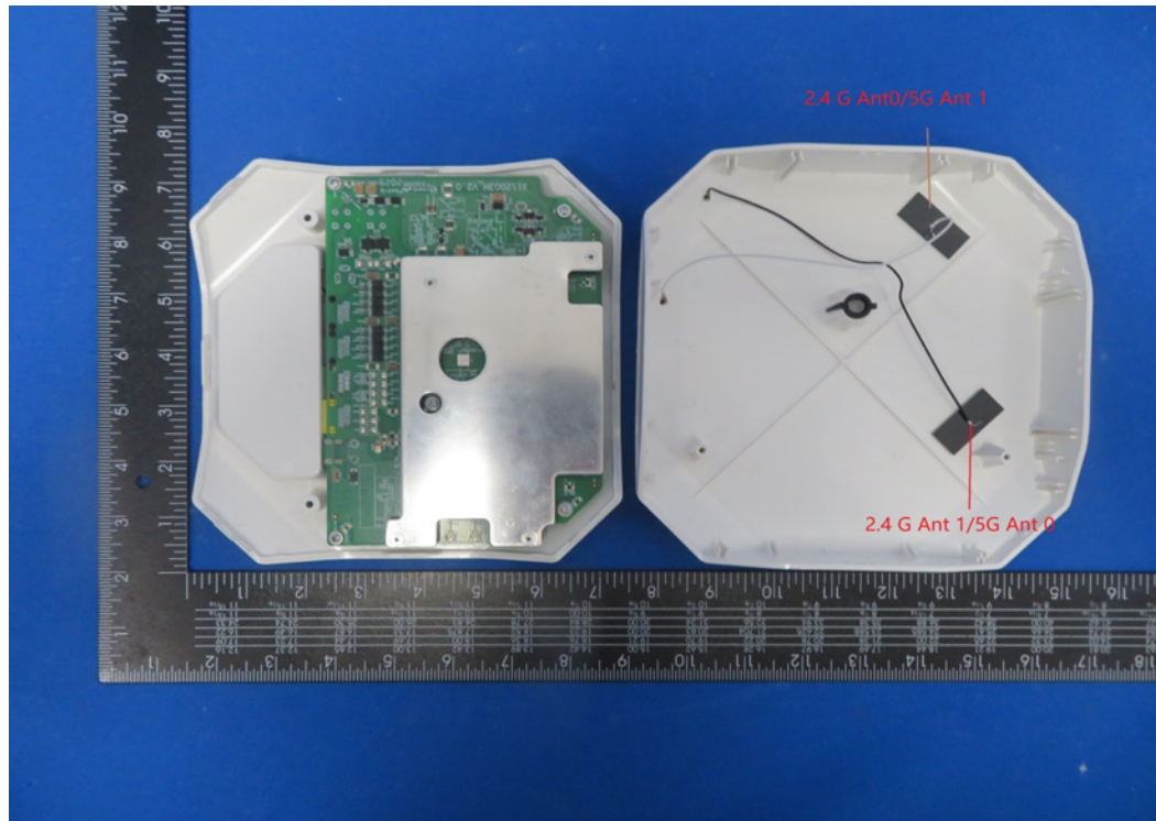
(1) EUT Photo
