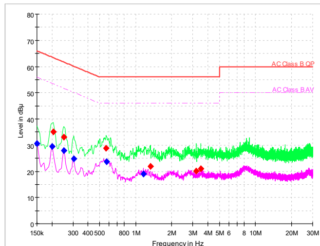
L+N Line
