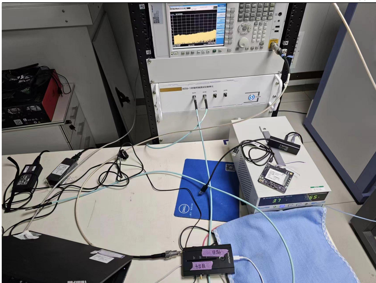
RF Conducted Test setup (BT)
