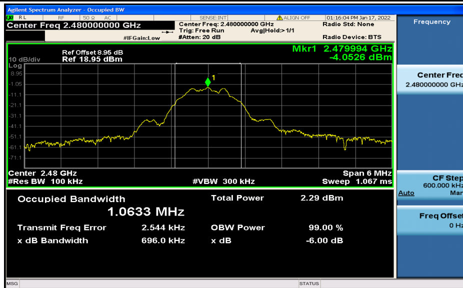
6dB Bandwidth_BLE_2480
