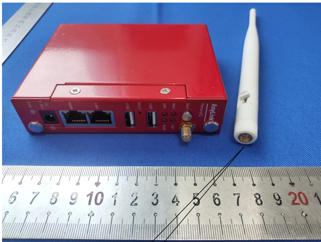
Model: NeuroQ
