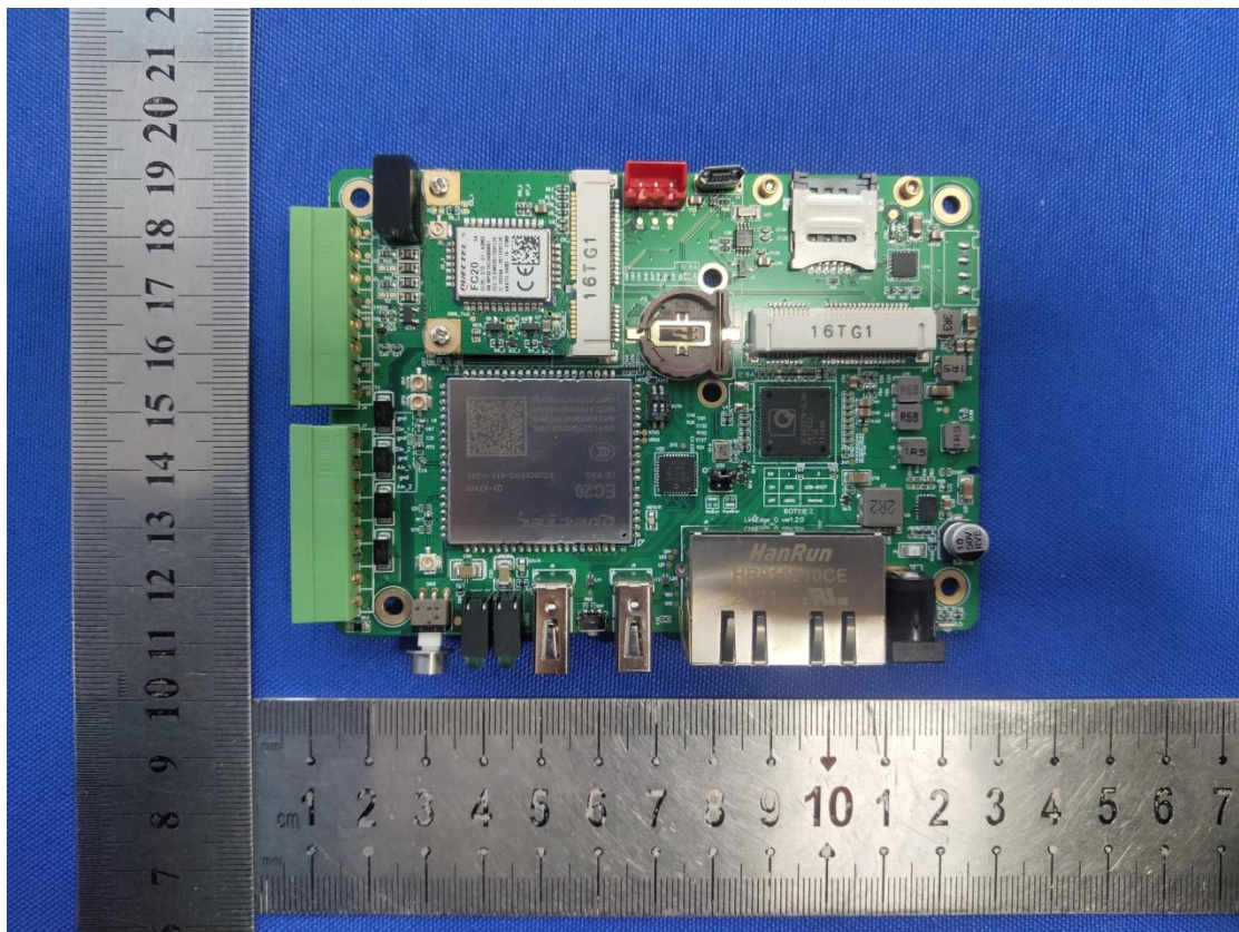
Model: NeuroQ
