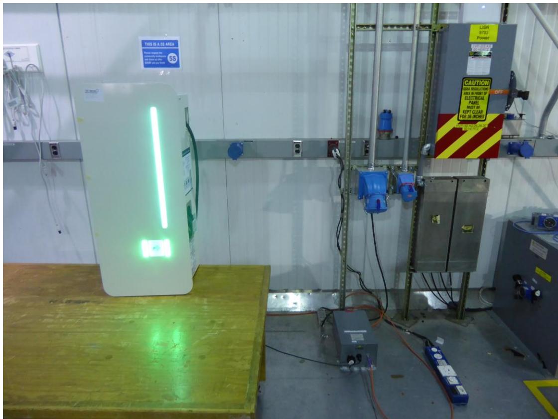
Figure 9 – Conducted Emissions Test Setup
