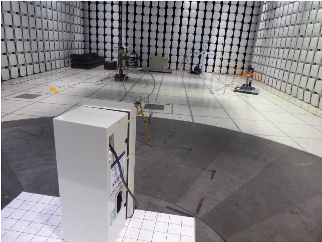
Figure 4 – 9k – 30MHz 3 meter Radiated Setup
