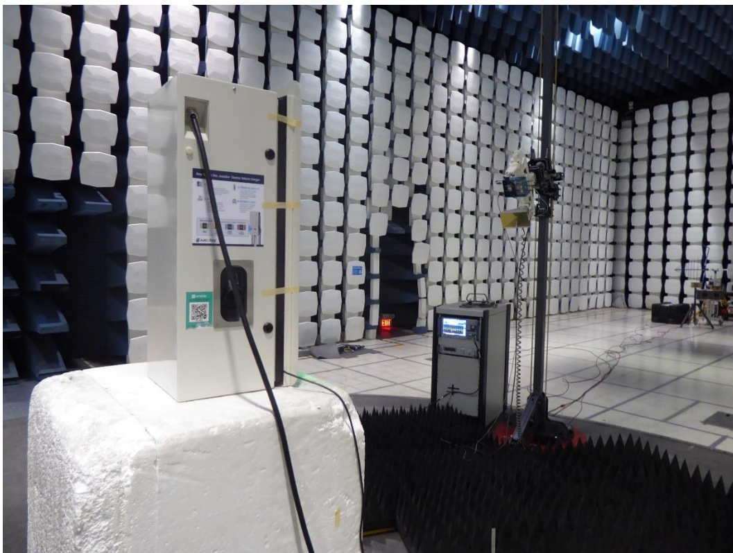
Figure 7 – 1 – 26.5 GHz 3 meter Radiated Setup
