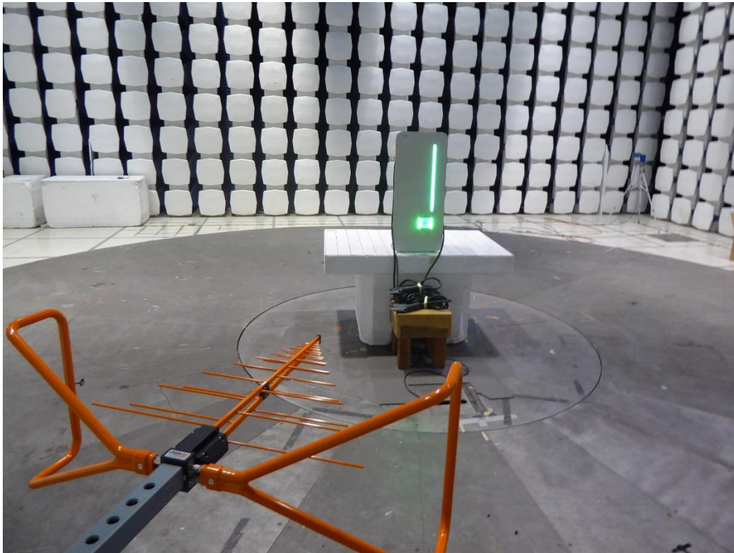
Figure 6 – 30 – 1000 MHz 3 meter Radiated Setup
