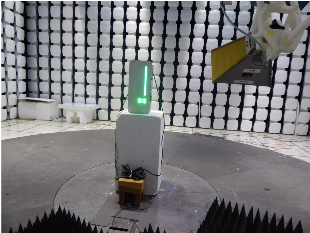
Figure 8 – 1 – 26.5 GHz 3 meter Radiated Test Setup
