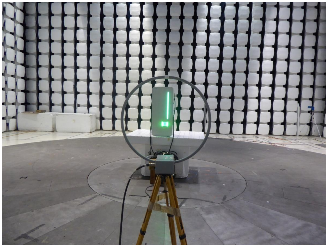
Figure 3 – 9k – 30MHz 3 meter Radiated Setup
