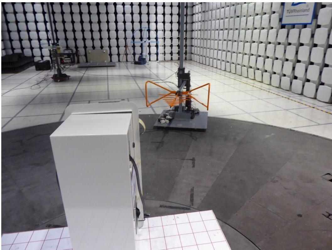
Figure 5 – 30 – 1000 MHz 3 meter Radiated Setup
