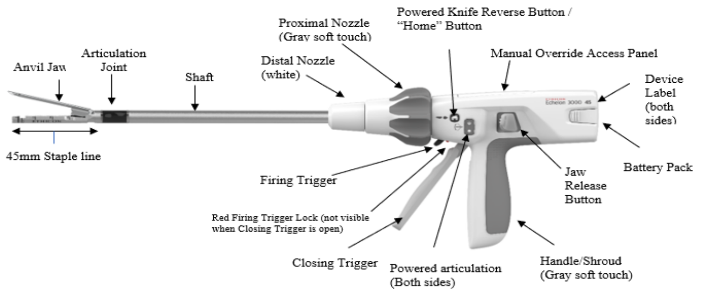
Figure 8: Echelon 3000 External Features
