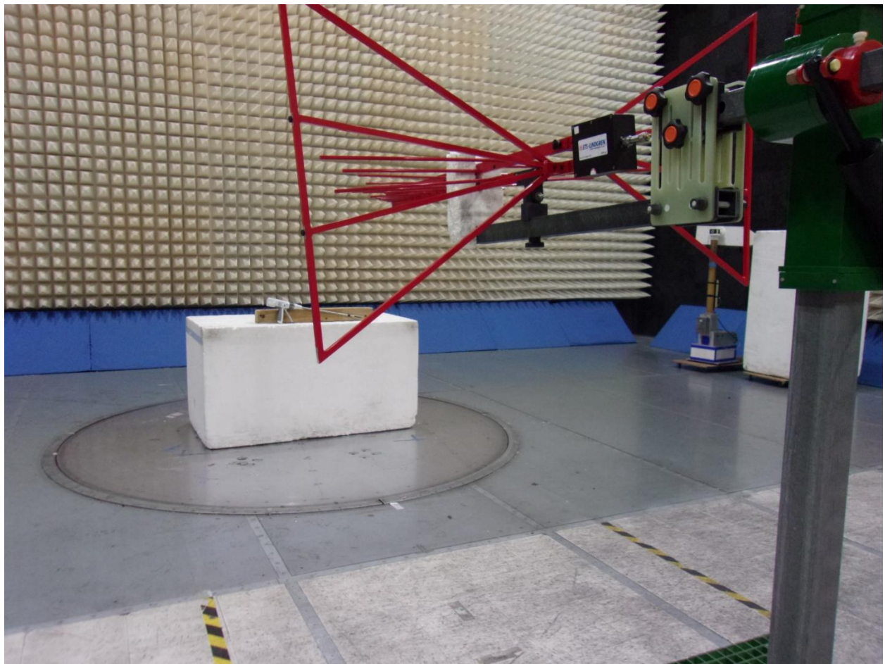
Figure 1 Unintentional and radiated spurious emissions, 30MHz – 1GHz
