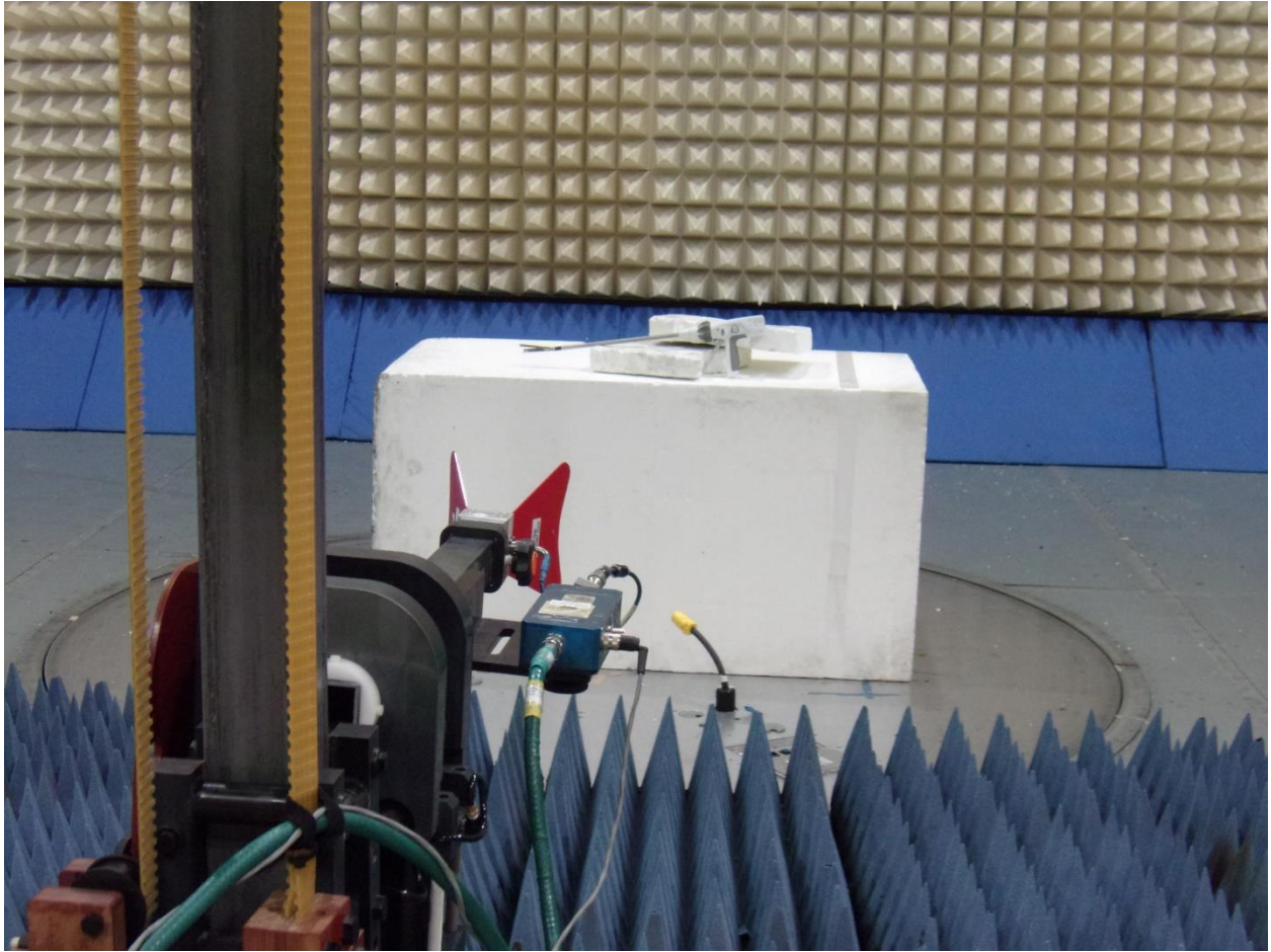
Figure 2 Unintentional emissions, 1GHz – 18GHz
