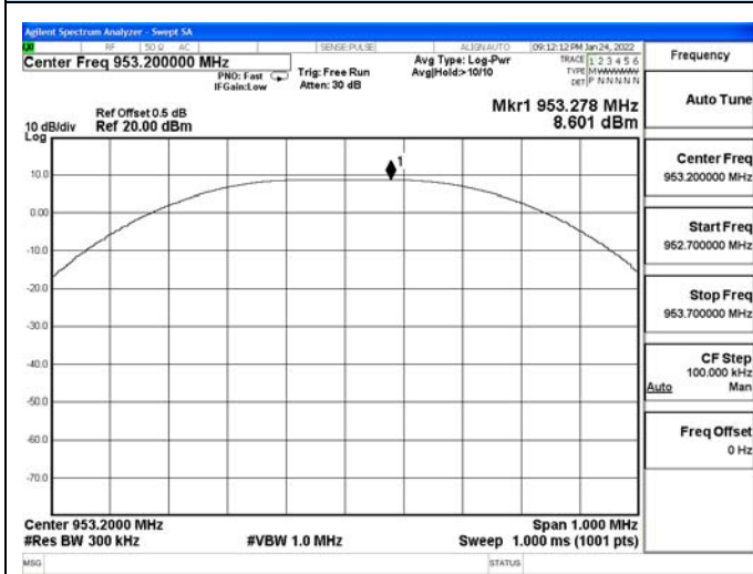
Channel 1 / 953.2 MHz
