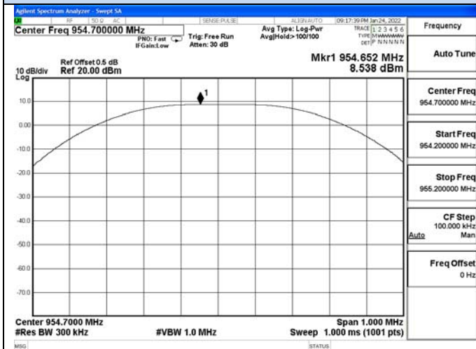
Channel 6 / 954.7 MHz
