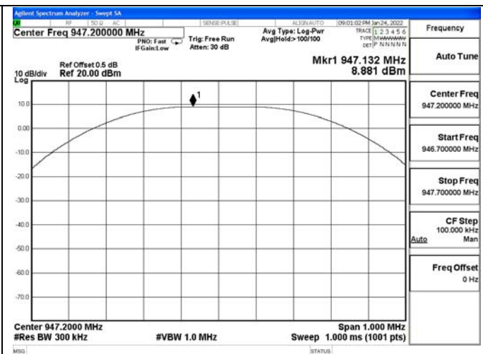
Channel 17 / 947.2 MHz
