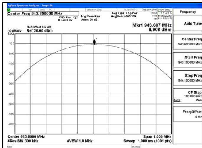
Channel 7 / 943.6 MHz
