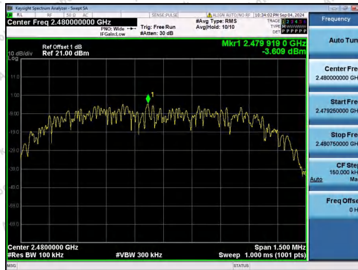
2D5-Ant1-2480-0~Reference-PASS
