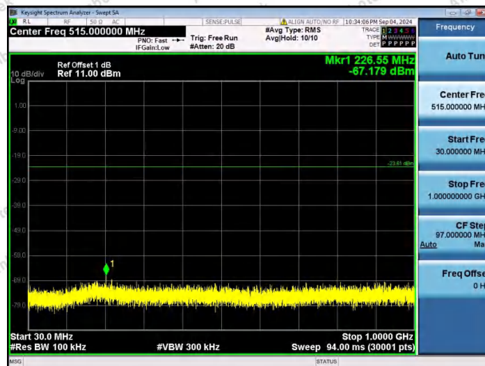
2D5-Ant1-2480-30~1000-PASS
