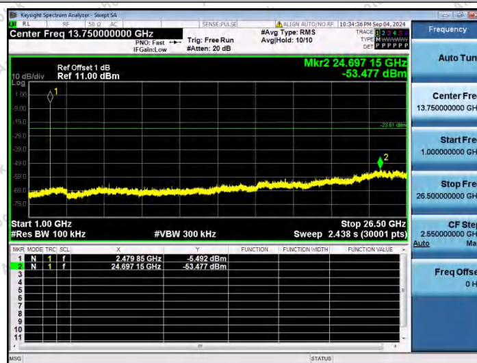
2D5-Ant1-2480-1000~26500-PASS
