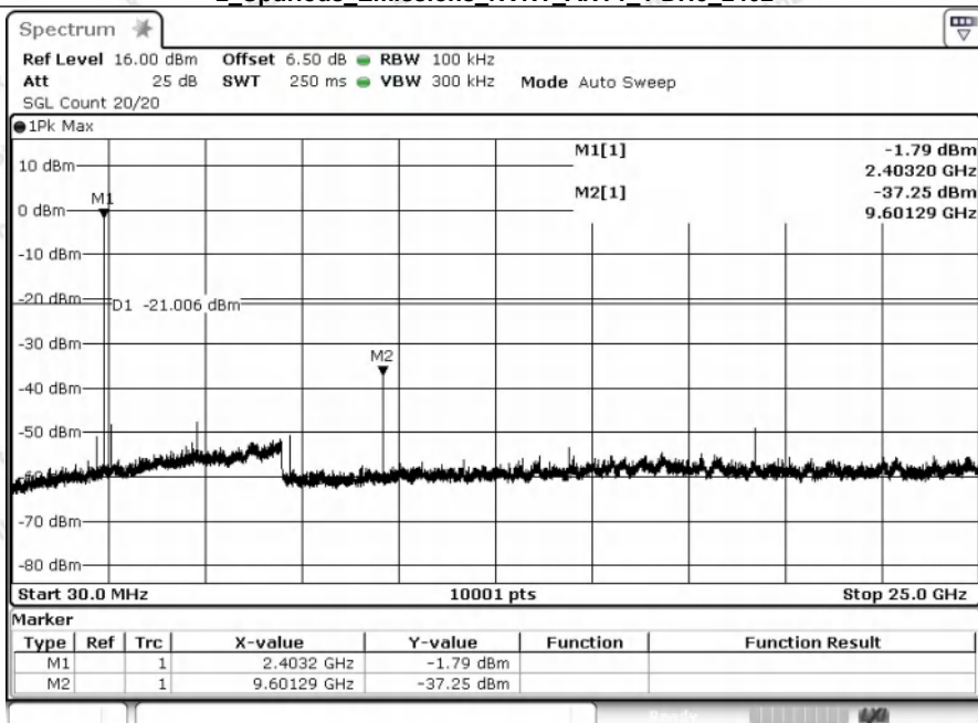
2 Spurious Emissions NVNT_ANT1_1-DH5_2402
