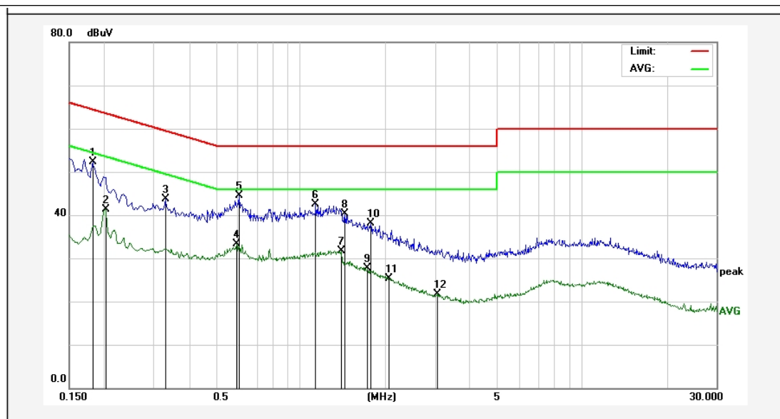
TM3 / Line: Neutral / Band: 2400-2483.5 MHz / BW: 1 / CH: L
