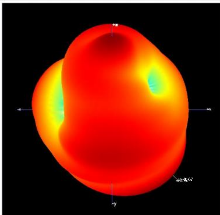
B1.3 3D Pattern for 2500MHz
