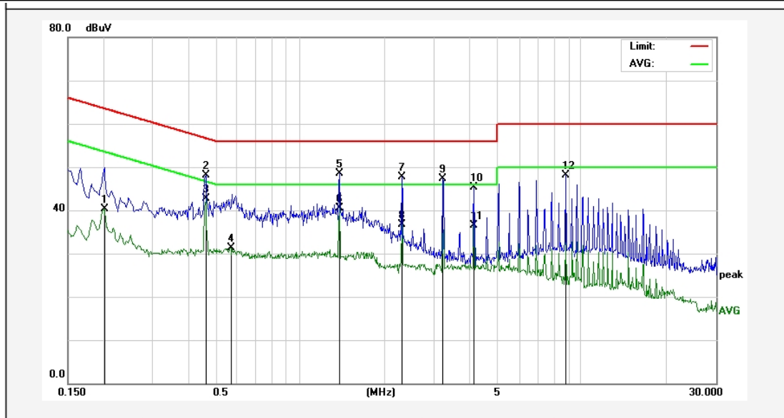
TM3 / Line: Neutral / Band: 2400-2483.5 MHz / BW: 1 / CH: L
