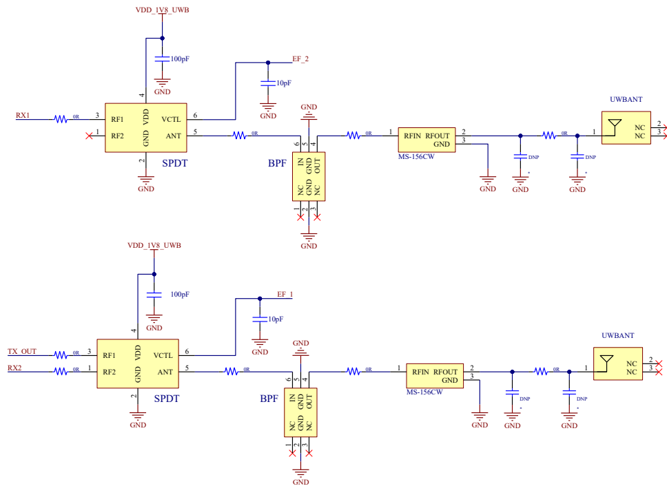
Figure 5 : UWB SR150 Module 2D AoA configuration
