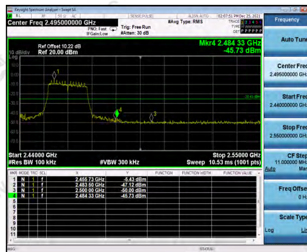
Right bandedge
