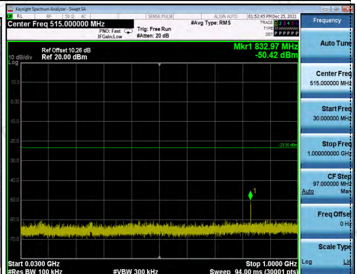
Reference CH06
