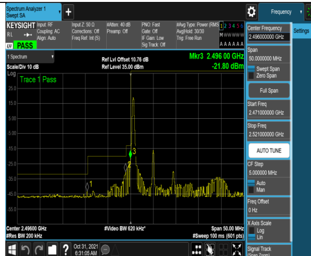
Band41-10MHz-16QAM-39700-1RB#49
