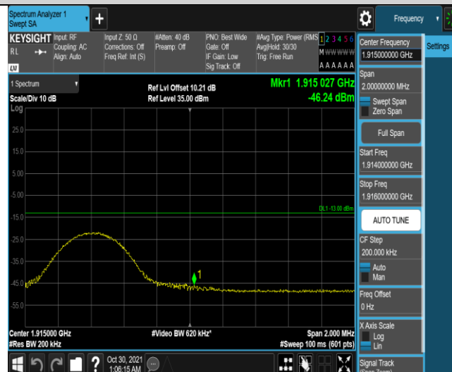
Band25-10MHz-16QAM-26640-1RB#49
