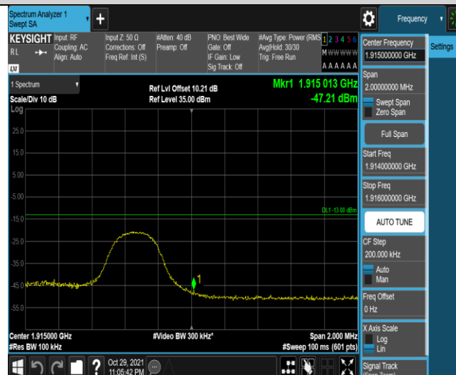
Band25-5MHz-QPSK-26665-1RB#24
