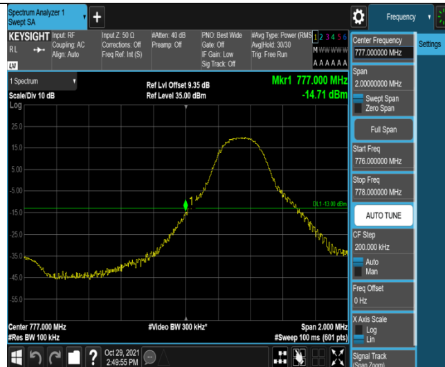
Band13-5MHz-16QAM-23205-1RB#24
