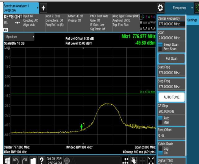
Band13-5MHz-16QAM-23205-25RB#0
