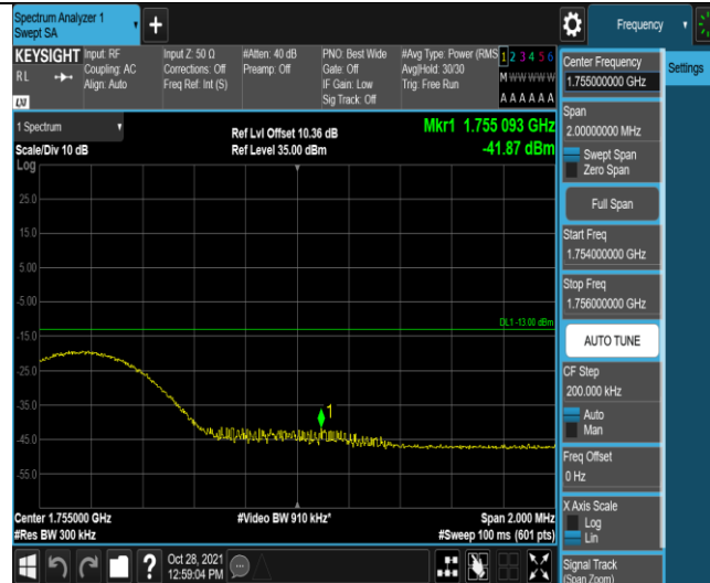
Band4-15MHz-16QAM-20325-1RB#74
