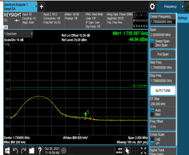
Band4-10MHz-QPSK-20350-1RB#49
