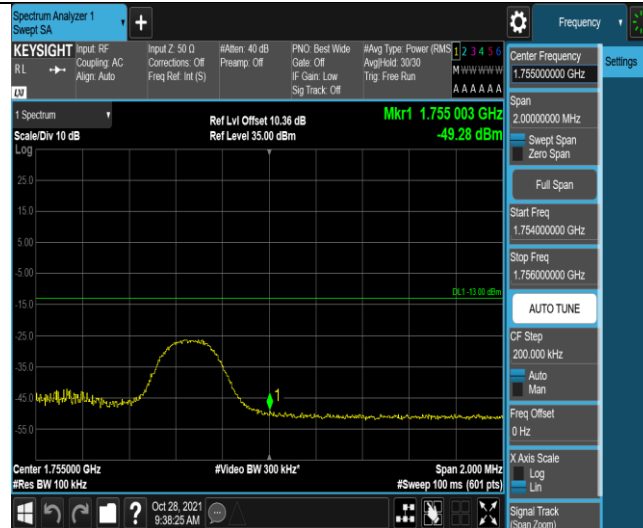
Band4-5MHz-16QAM-20375-1RB#24
