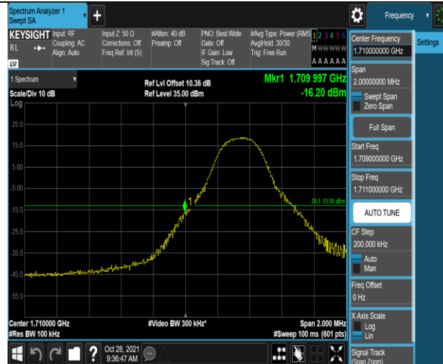
Band4-5MHz-16QAM-19975-1RB#24
