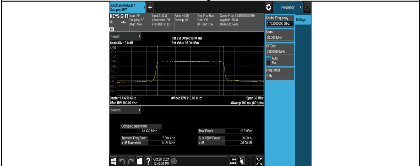
Band4-15MHz-16QAM-20325-75RB#0
