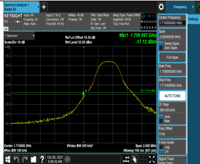
Band4-5MHz-QPSK-19975-1RB#24
