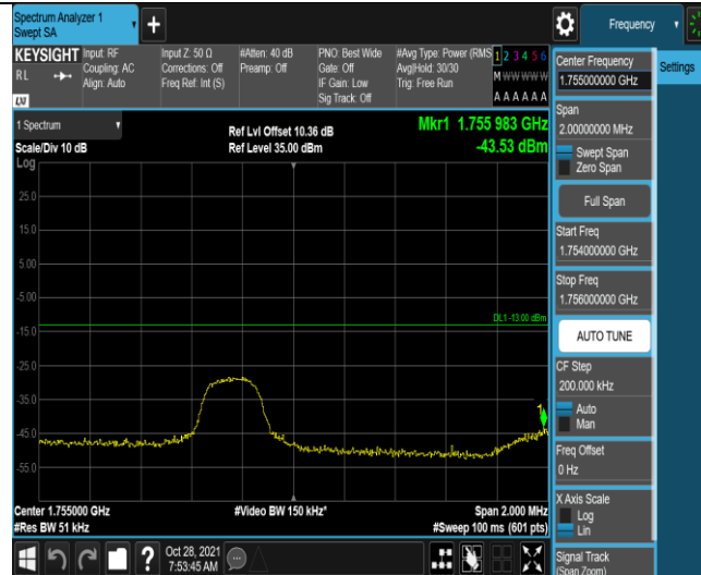
Band4-3MHz-QPSK-20385-1RB#14
