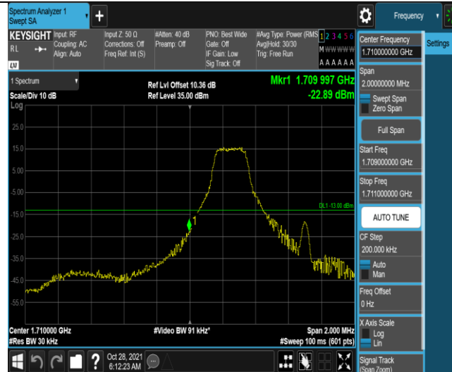
Band4-1.4MHz-16QAM-19957-1RB#5
