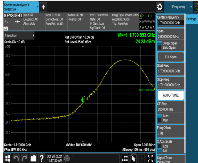
Band4-10MHz-QPSK-20000-1RB#49
