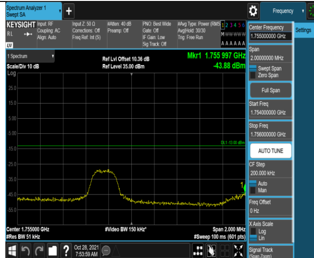
Band4-3MHz-16QAM-20385-1RB#14
