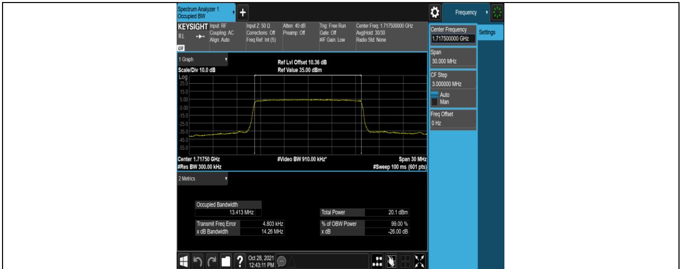
Band4-15MHz-16QAM-20175-75RB#0
