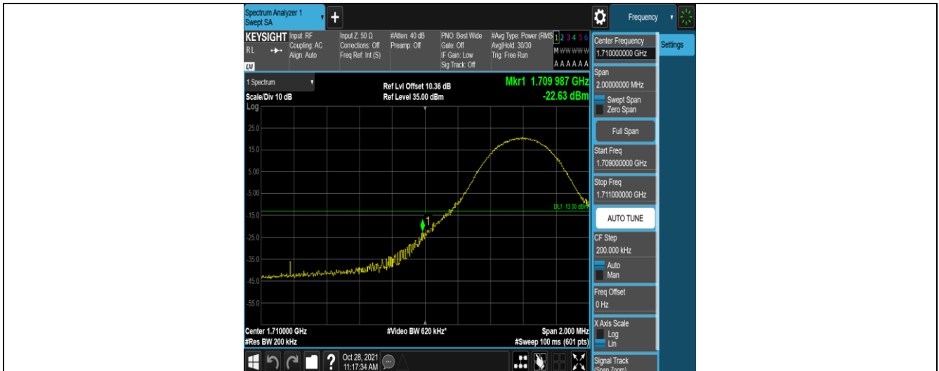
Band4-10MHz-16QAM-20000-1RB#49
