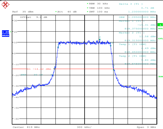
Band26-1.4MHz-QPSK-26740-6RB#0
