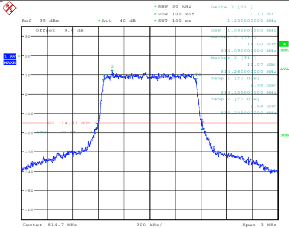
Band26-1.4MHz-QPSK-26697-6RB#0
