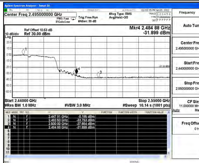
11N40SISO_Ant_High_2452_Peak
