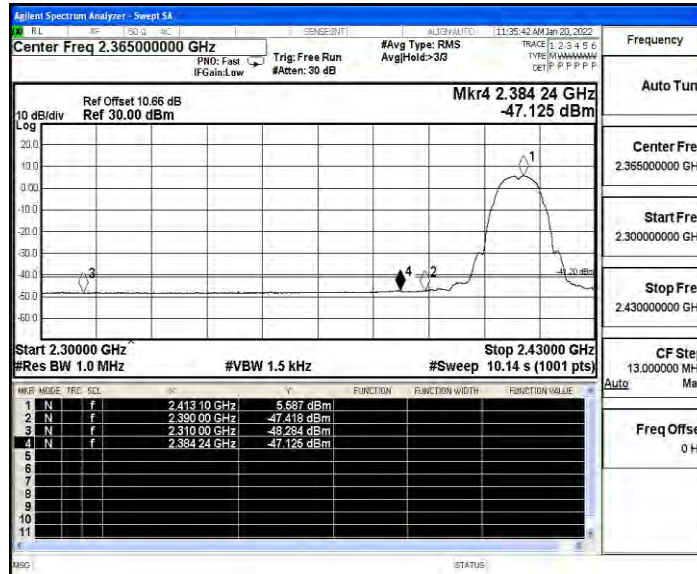
11B_Ant_Low_2412_Peak
