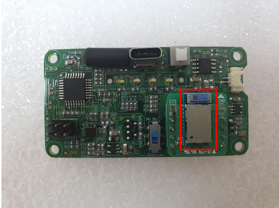
(Without shield can)Antenna & Granted Module(FCC ID : 2APB6-BOT-NLE521)
